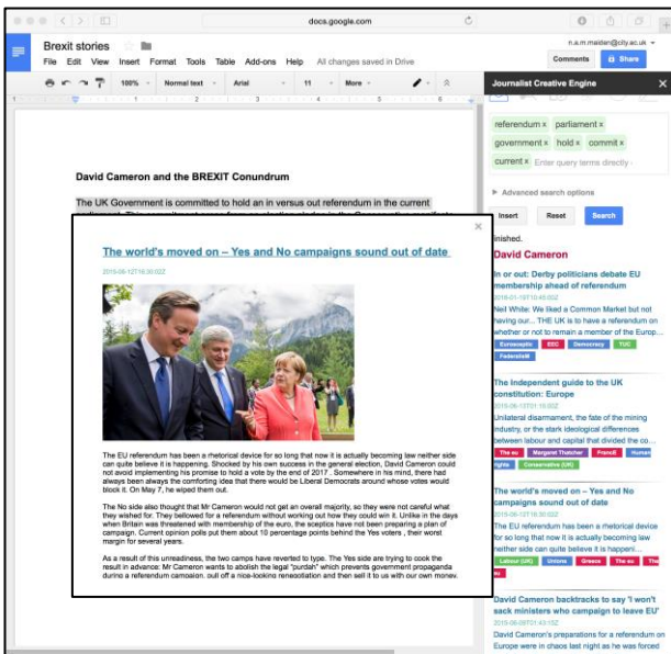
Figure 4: JUCE showing creative search results retrieved for the inserted text (about David Cameron) in the sidebar, and one story in the opened dialogue box
