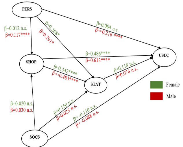
Figure 3. Path coefficient and significance between females and males. PERS = personality, SHOP = shopper type, SOCS = Social support, STAT = Need for status, USEC = Continuance intention. n.s. = Not significant
