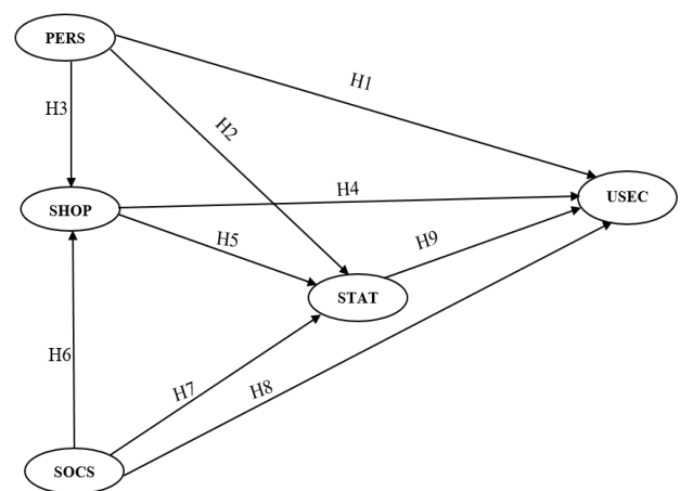
Figure 1. Research model. All paths assumed positive. PERS = Personality, SHOP = Shopper type, SOCS = Social support, STAT = Need for status, USEC = Continuance intention
